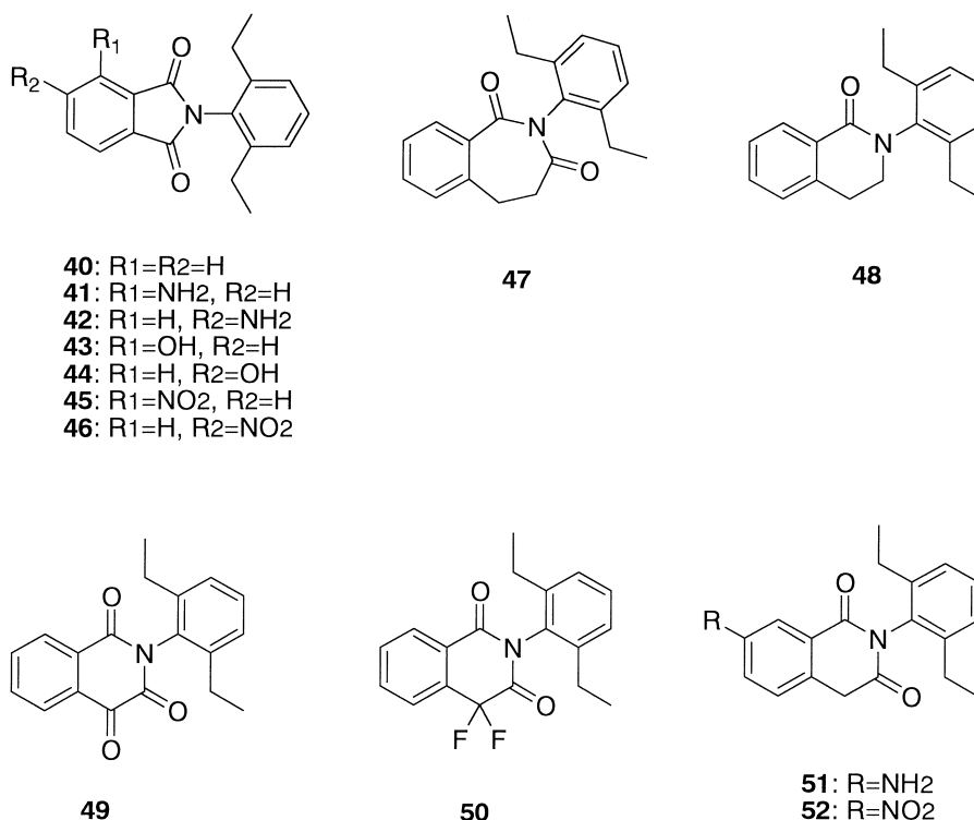
Figure 5. Structures of some derivatives of PIQ-22.
